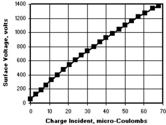
Figure 4: Charging of a 31 cm 2 silicate glass sample by 10 keV electrons.
