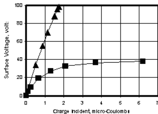
Figure 3: Sample voltage vs. incident charge from the electron filament that was attracted to the sample surface by +100 V on the rear electrode.
