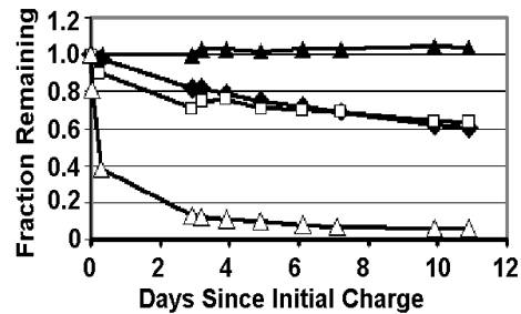
Figure 5: Surface voltage decay for three silicate glass samples and one FR4 PC board sample (lower).
