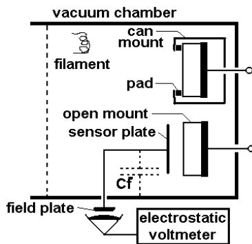
Figure 2: The floating voltmeter, and two sample mounts: open and covered.
