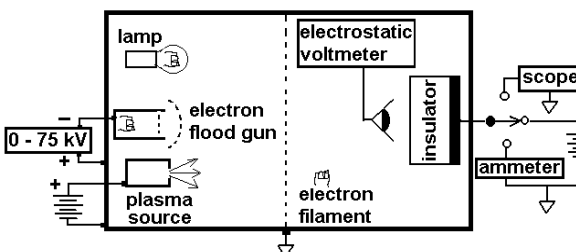
Figure 1: Depiction of an insulator sample that may alternately be exposed to various environments and electrical measurements.
