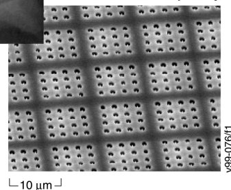
b. Portion of 10,000-tip array
