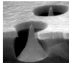
a. Close-up of single tip
