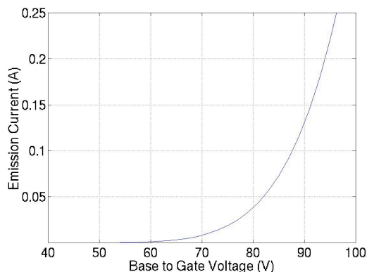
Figure 4. Modeled values of emitted current vs. gate voltage for 5-million-tip Spindt cathode.
