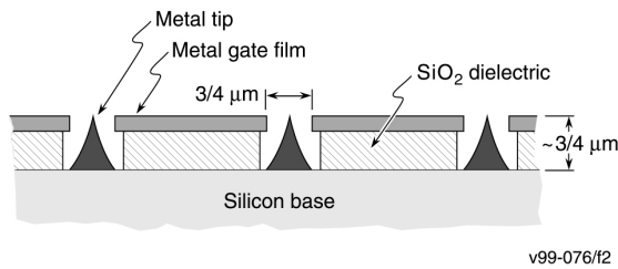
Figure 3. Schematic of a Spindt cathode array.
