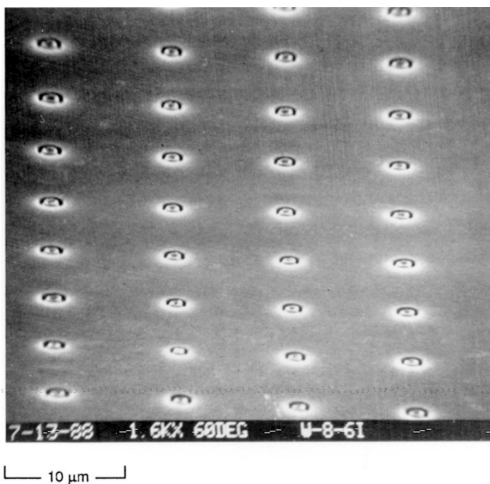
Figure 5. Electron micrograph of one type of field ionization array.
