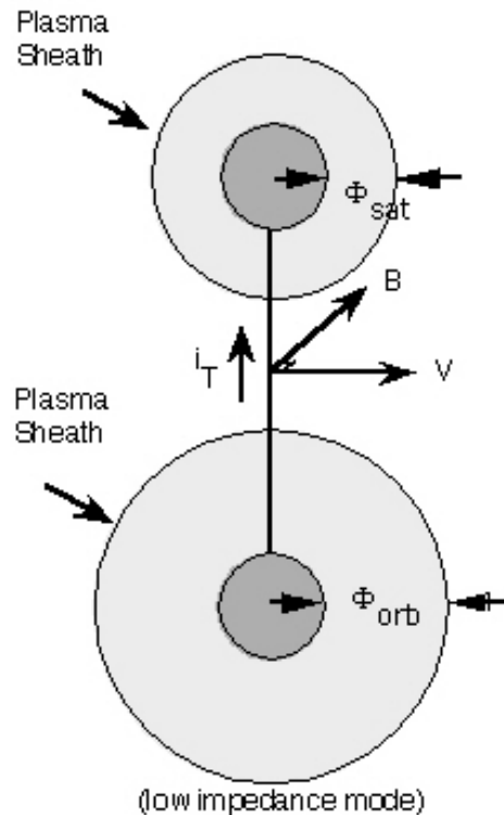
Figure 6. Schematic of an electrodynamic tether system flowing current.
