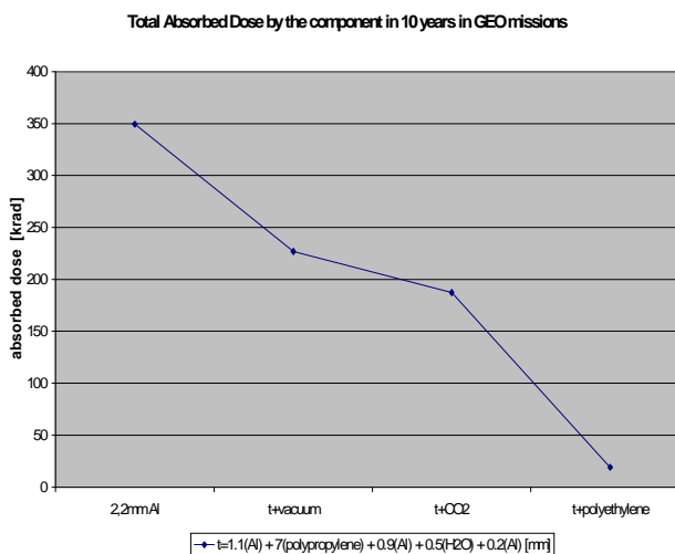
Fig.17- Total Absorbed Dose for a NEGESAR-based Equipment in GEO missions
