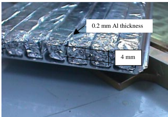
Fig.13- Contact conditions of the Filler
