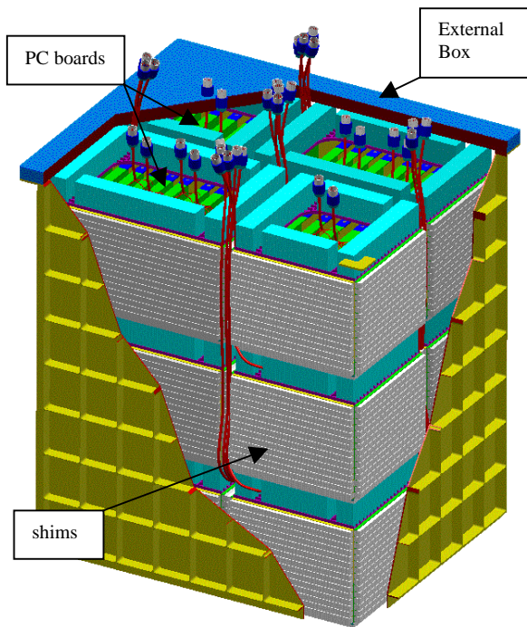
Fig.4- Typical layout of a microsatellite based on the NEGESAR Tecyhnoogy
