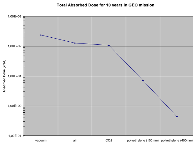
Fig.5- Electrons and Protons absorbed total dose in function of different shielding materials
