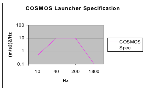
Fig.8- COSMOS Launcher Specification
