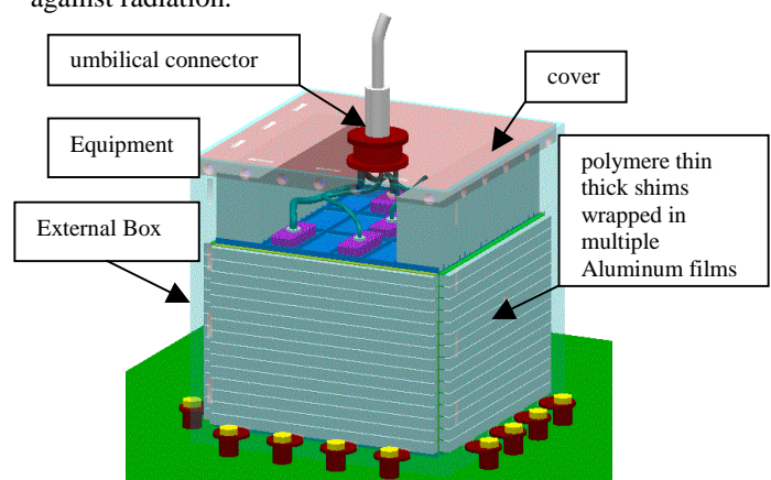
Fig.1 – Single Equipment configuration
