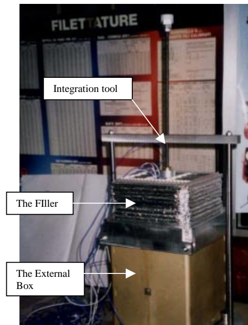
Fig.6- The SMALL DEMONSTRATOR in the integration phase
