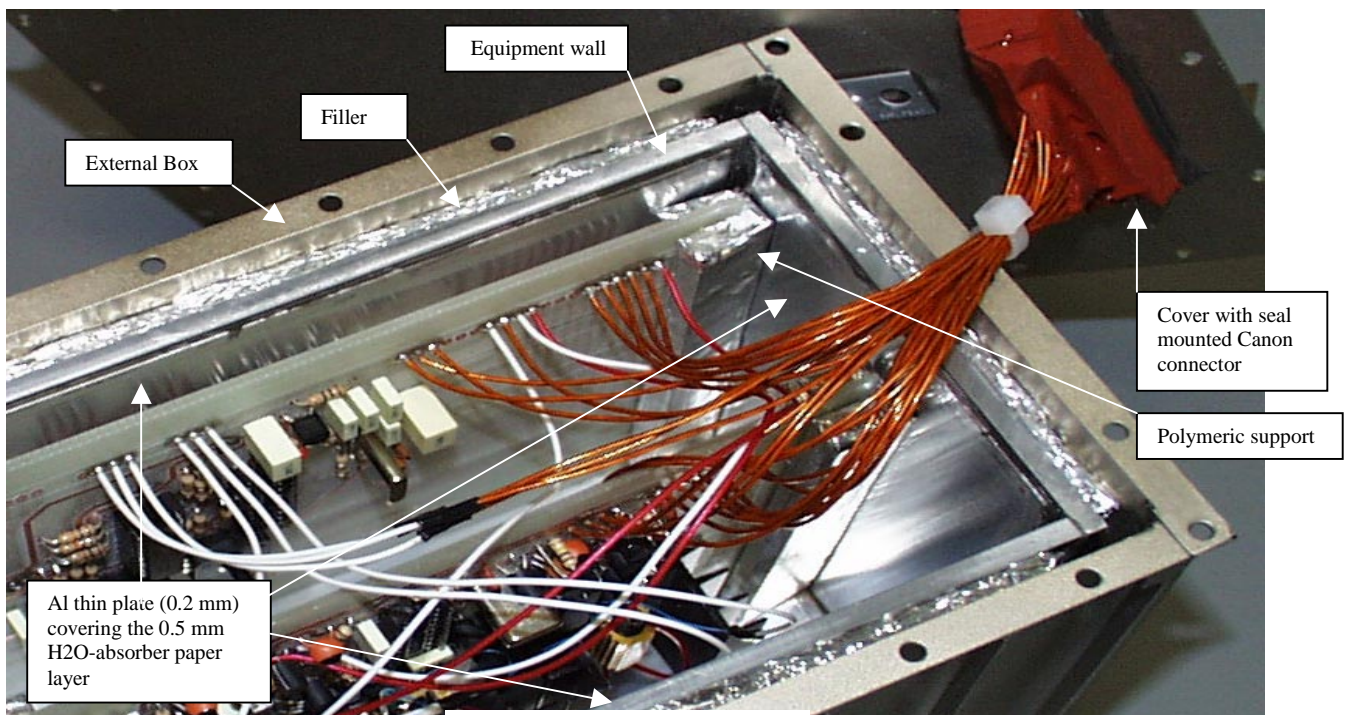
Fig.15- SOFTEQ (SOFT Equipment)
