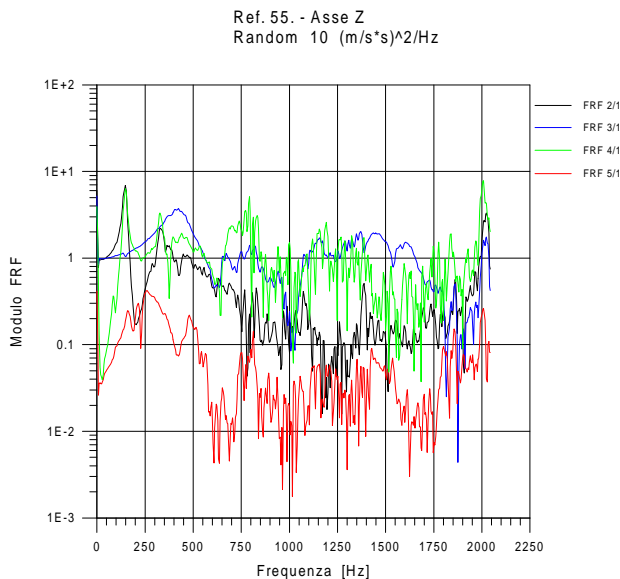
Fig.9- Random Test on the Z axis.
