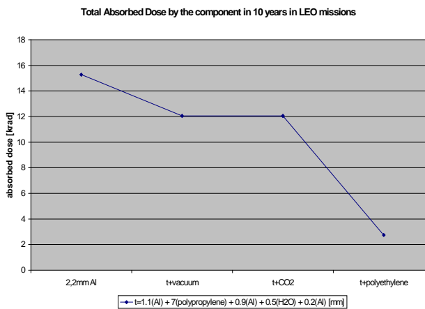
Fig.16- Total Absorbed Dose for a NEGESAR-based Equipment in LEO missions
