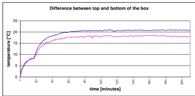
Fig.11- \Delta T in the case of empty box.
