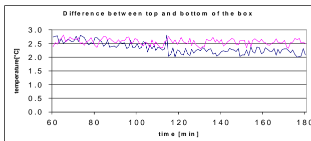
Fig.12- \Delta T with Filler wrapped in 2 (0.03 mm) and 7 (0.105 mm) Aluminium layers
