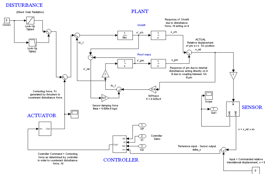
Figure 3 : Schematic of Translational Control-Loop for One Axis
