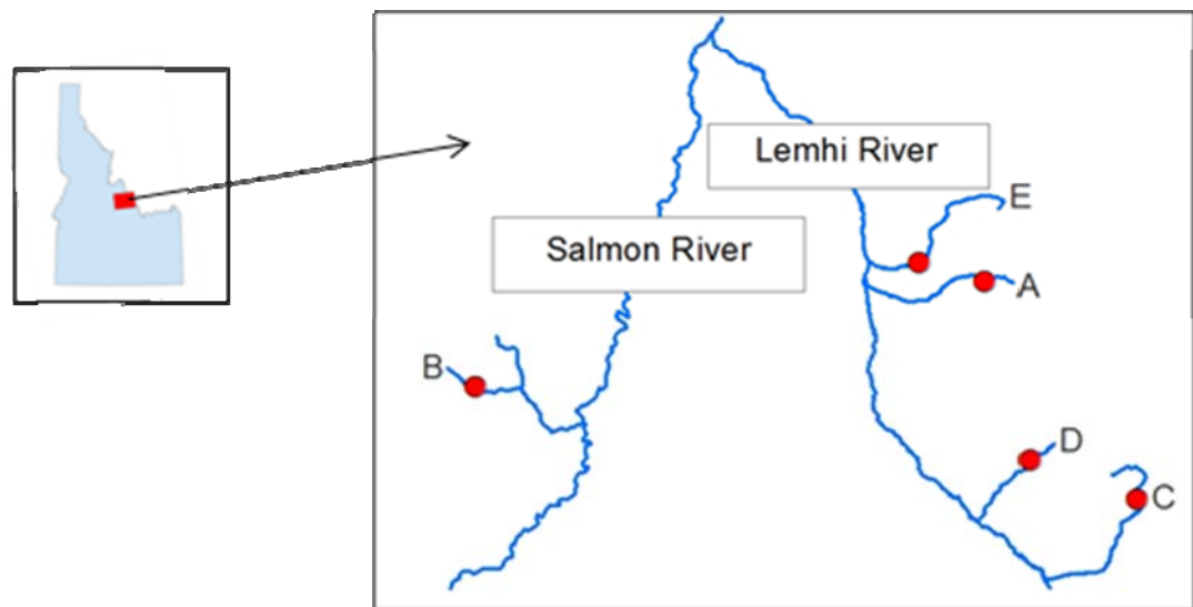
Fig. 1. Streams included in this study were (A) Agency, (B) Big Hat, (C) Canyon, (D) Little Eightmile, and (E) Pattee.
