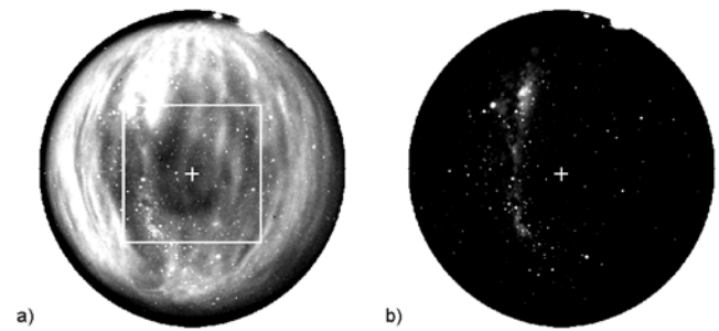
Figure 1. All-sky image (a) in sodium emission and (b) at a background wavelength, shown on the same gray scale range for the night of 20–21 July 2001. North is at the top and east to the right of the images, and the approximate 150-km field of view analyzed is shown on the Na image. Gravity wave structures aligned N-S, and moving toward the west, are apparent in the Na airglow image, while the stellar and galactic backgrounds that must be removed before processing are more obvious in the background image.
