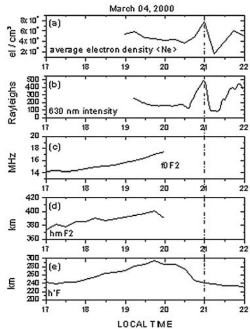
Figure 5. (a) Calculated bottomsides average electron density; (b) OI 630 nm zenith intensity; (c) critical frequency of the F-layer ( f_oF2 ); (d) F-region peak height ( h_mF2 ); and (e) F-region minimum virtual height ( h'F ). Data obtained on March 04, 2000, near the equatorial anomaly southern crest, showing the occurrence of plasma density enhancement, or blob around 21 LT.
