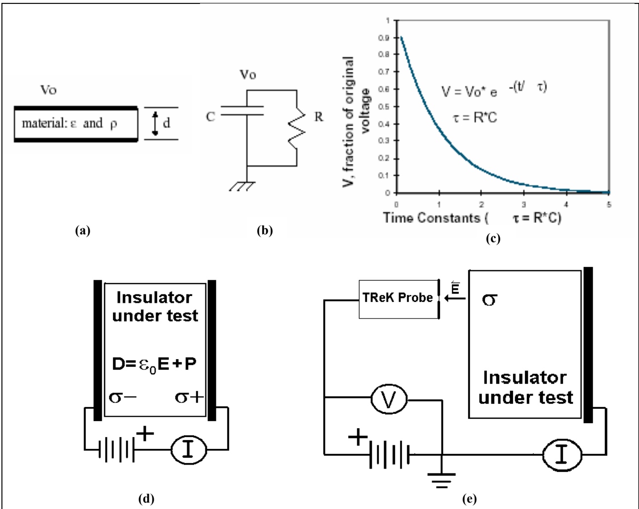
Figure 2. Resistivity can be measured using the simple RC time constant method. (a) Simple thin film capacitor sample geometry with thickness d , surface area A , permittivity \epsilon , and resistivity \rho = R \cdot A/d , where R is the sample resistance. (b) Schematic of a simple RC test circuit with sample capacitance C and resistance R of a sample with surface voltage V(t) = V_0 e^{-t/\tau} as a result of stored charge \sigma(t) = \sigma_0 e^{-t/\tau} . (c) A typical decay curve of sample voltage as a function of time, t , with time constant \tau = R \cdot C = \epsilon \cdot \rho . (d) Schematic of Capacitor (Constant Voltage) Resistivity Test Circuit. (e) Schematic of Charge Storage Resistivity Test Circuit.
