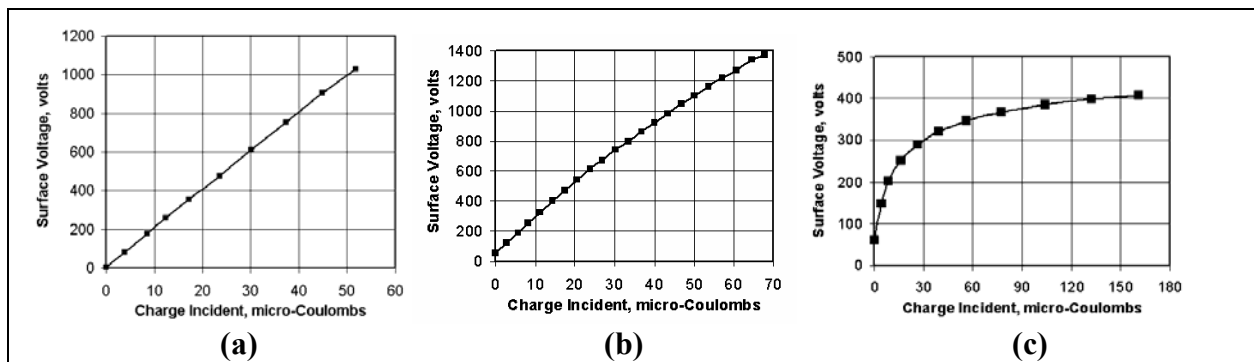
Figure 8. Effect of high-energy electron bombardment on charge storage. Q-V electron-beam charging data for three similar 25 \mu\text{m} (proprietary undisclosed materials) silicate glass samples [also shown in Figure 4(a)]. Q is the cumulative charge incident on the sample surface from a series of short high-energy electron beam bursts and V is the measured incremental surface voltage proportional to surface charge. (a) 10-keV charging curve for non-leaky sample, where the electron penetration depth was less than 10% into the insulator and the E-field at the rear of the insulator was relatively small. (b) 10-keV charging curve for slightly leaky sample. (c) Charging curve of a similar sample using 40-keV incident electrons, where the electron penetration depth was nearly 90% into the insulator and the E-field at the rear of the insulator was relatively large [4].
