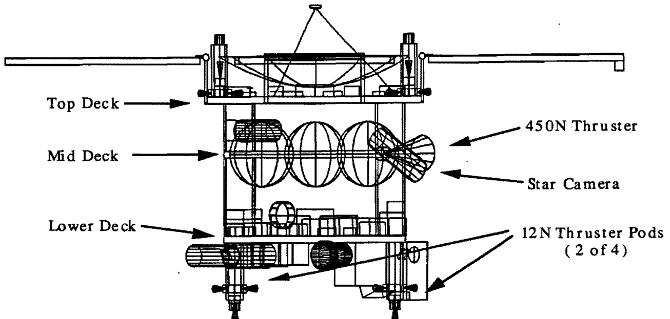
Figure 6 - Spacecraft Layout
