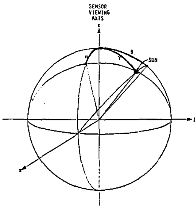
Figure 2. Sun's spherical coordinates in sensor's coordinate system
