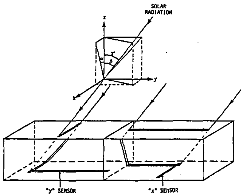
Figure 3. Schematic showing separation of sun's rays into x and y components
