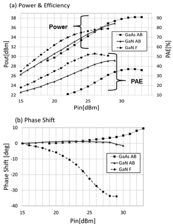
Figure.5: Comparison of three types of X-band RF power amplifiers. GaAs FET of AB class, GaN HEMT of AB class, and GaN HEMT of F class. (a) output power and power-added efficiency vs. input power. (b) phase shift vs. input power.
