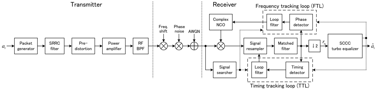
Figure.14: System block diagram of high-data-rate downlink including satellite segment (left) and ground station (right).
