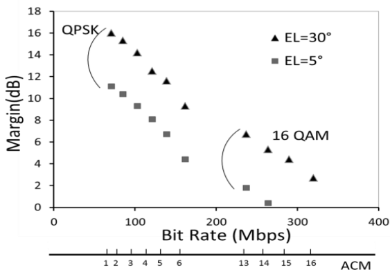
Figure.4: Link margin of high-data-rate down link as function of data bit rate or ACM number. Symbol rate is 100MSPs, and elevation angle is 30° and 5°. Altitude is 600km and 13.5dBi MGA is applied. RF power amplifier is GaN HEMT of AB class with 26dBm input.
