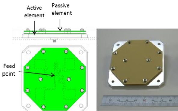
Figure.9: Structure and photograph of medium gain antenna with four active arrays and four passive arrays. Mass is 150g and size is 70 x 70 x 10mm 3 .
