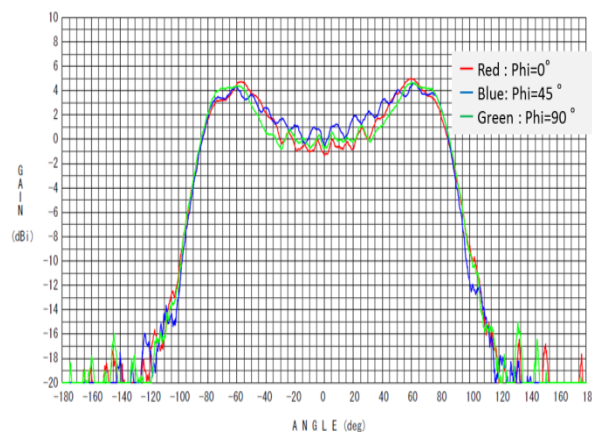
Figure.12: Measurement results of iso-flux antenna pattern with quadrafilax helix elements ( \alpha=20^\circ , D=10\text{mm} , H=20\text{mm} ). Horizontal axis is angle from antenna normal plane. Phi is azimuthal angle. Frequency : 8160MHz.
