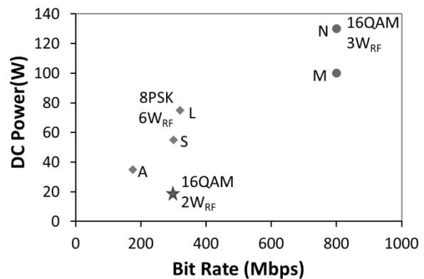
Figure 1: DC power consumption vs. data bit rate for onboard high-data-rate transmitter. ◆ and ● correspond to conventional transmitters with 8PSK and 16QAM, respectively. ★ denotes our novel transmitter with 16QAM. RF power levels are also indicated.
