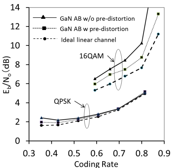
Figure.16: Simulation results of required E_b/N_o for 16QAM and QPSK as function of ACM coding rate. Broken line: ideal linear channel. Also E_b/N_o for GaN HEMT AB class amplifiers of 26 dBm input are shown. Solid line: without pre-distortion. Dotted line: with pre-distortion.
