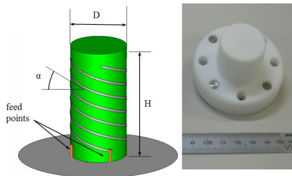
Figure.11: Structure and photograph of iso-flux antenna with quadrafilax helix elements. Mass is 150g, \alpha=20^\circ , D=10\text{mm} , H=20\text{mm} .
