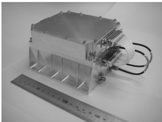
Figure.7: Photograph of engineering model of high-data-rate X-band 16QAM transmitter. Maximum data rate is 348 Mbps, RF output is 2W, DC power is 18W, and mass is 1330g and size is 120 x 120 x 73 mm 3 .
