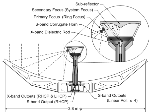
Figure.13: Structure of compact S/X dual band Cassegrain antenna with 3.8m diameter.
