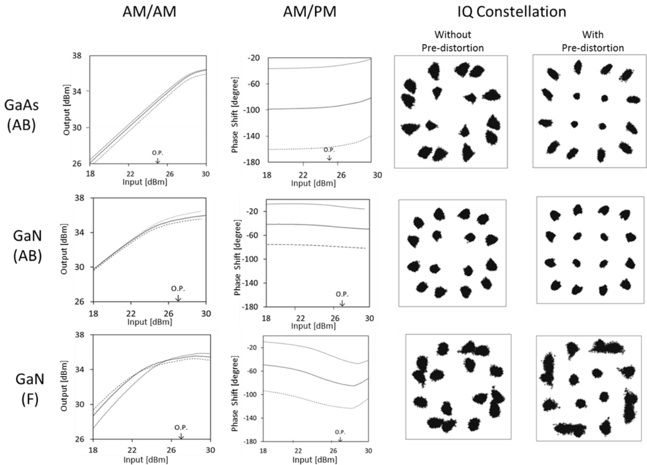
Figure.6: Nonlinearities of RF power amplifiers and their effects on IQ constellations for 16QAM. Amplifiers are GaAs FET amplifier of AB class (25dBm input), GaN HEMT amplifier of AB class (27dBm input), and GaN HEMT amplifier of F class (27dBm input). Nonlinearities are experimentally measured for 100MHz frequency bandwidth in terms of amplitude (AM/AM) and phase (AM/PM) characteristics. Thin line: 8150 MHz, thick line: 8200MHz, dotted line: 8250MHz. IQ constellations without pre-distortion and with memoryless pre-distortion are obtained by SPW simulation. Operating points (input power level) of amplifiers are shown by O.P.
