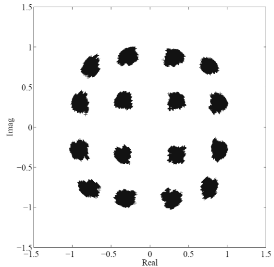
Figure.8: Measured IQ constellation of engineering model of transmitter with GaN HEMT amplifier of AB class. Symbol rate is 100Mps. RF output is 33dBm.
