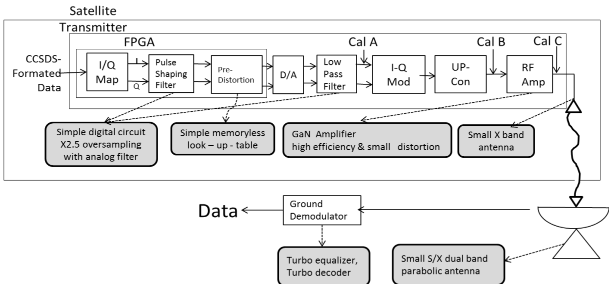
Figure.3: System block diagram of high-data-rate downlink. Several improvements are applied to satellite segment and ground segment.
