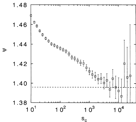
FIG. 3. Values of \psi obtained from fits to \mu_s^{(1)} = D_0 s^\psi for s \geq s_c as a function of s_c . The dashed line gives the presumed exact value \psi = \frac{127}{91} \approx 1.396 .
