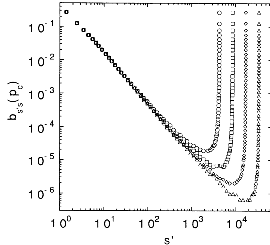
FIG. 4. Computed daughter distribution b_{s's}(p_c) for two-dimensional bond clusters as a function of the daughter mass s' plotted for parent masses s in the ranges 4096–4467 ( \circ ), 8192–8933 ( \square ), 16384–17867 ( \diamond ), and 32768–35734 ( \triangle ).
