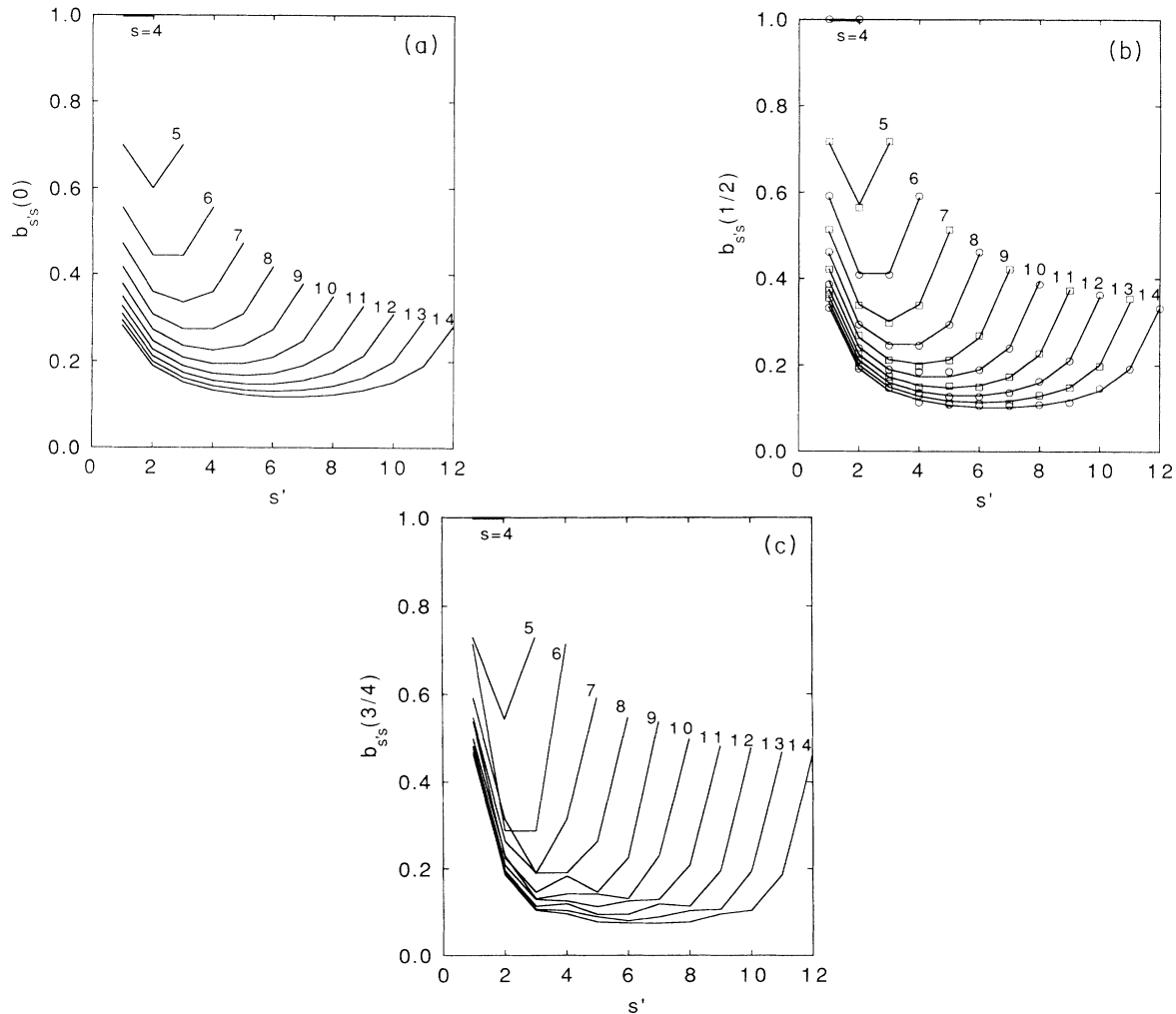
FIG. 12. Exact fraction b_{s's}(p) of daughter clusters of mass s' produced by the fragmentation of a parent cluster of mass s , for s=4, 5, 6, \dots, 14 at (a) p=0 , (b) p=\frac{1}{2} , and (c) p=\frac{3}{4} ; line segments connect adjacent values of b_{s's}(p) with the same values of s . These data show a deepening of the minimum of b_{s's}(p) with increasing p . Monte Carlo results are shown as data points in (b) for comparison; uncertainties in these results are smaller than the width of the plotting symbols.
