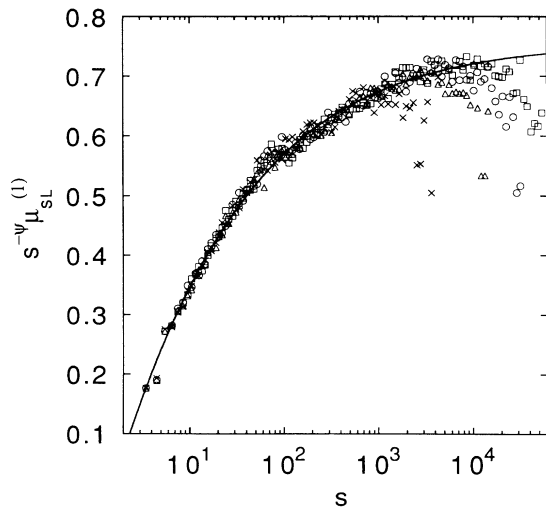
FIG. 6. Computed results (data points) for the scaled first moment s^{-\psi} \mu_{sL}^{(1)} = s^{-\psi} \sum_{s'=1}^{(s-1)/2} s' c_{s'sL}(p_c) of the ensemble average number c_{s'sL}(p_c) of daughters of mass s' on clusters of mass s on finite lattices of linear dimensions L = 100 ( \times ), 200 ( \triangle ), 300 ( \circ ), and 400 ( \square ) at p = p_c . The solid trace gives the fit to the infinite-lattice data (Fig. 2).
