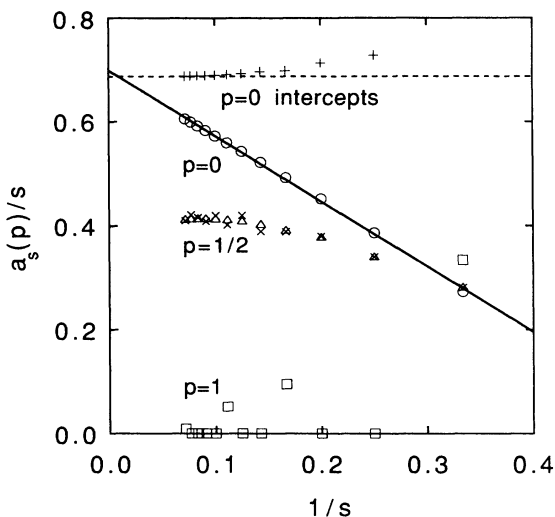
FIG. 11. Exact probability a_s(p)/s that removing a bond will break an s cluster as a function of 1/s , for p=0 ( \circ ), \frac{1}{2} ( \triangle ), and 1 ( \square ). The solid trace is a linear fit to the p=0 data, with intercept a_s(0)/s=0.70 for s \rightarrow \infty . Also shown are extrapolated intercepts from pairwise fits to these data ( + symbols plotted at the lower 1/s value of each pair), along with a dashed horizontal line at a_s(0)/s=0.69 through the fit to the two largest values of s . Monte Carlo data are shown for p=\frac{1}{2} ( \times ) for comparison; uncertainties in these results are comparable to the width of the plotting symbols.
