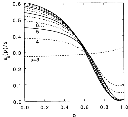
FIG. 10. Exact probability a_s(p)/s that removing a bond will break an s cluster as a function of p , for 3 \leq s \leq 14 .
