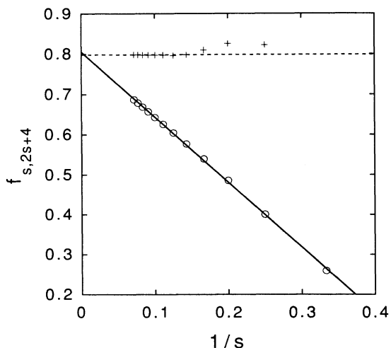
FIG. 9. Exact probability f_{s,2s+4} ( \circ ) that removing a bond from a cluster of mass s and maximum perimeter t=2s+4 will break the cluster as a function of 1/s . The solid trace is a linear fit to the data, with intercept 0.81. Also shown are extrapolated intercepts from pairwise fits to the data ( + symbols plotted at the lower 1/s value of each pair), along with a dashed horizontal line at f_{s,2s+4}=0.80 through the pairwise fit for the two largest values of s . The data indicate that f_{s,2s+4} < 1 even as s \rightarrow \infty .
