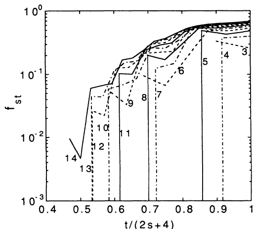
FIG. 8. Exact probability f_{st} that removing a bond from a cluster of mass s and perimeter t will break the cluster as a function of the scaled perimeter t/(2s+4) , where 2s+4 is the maximum perimeter, for s=3,4,5, \dots, 14 (numerical labels). The data raise the question of whether a scaling form exists for large s .
