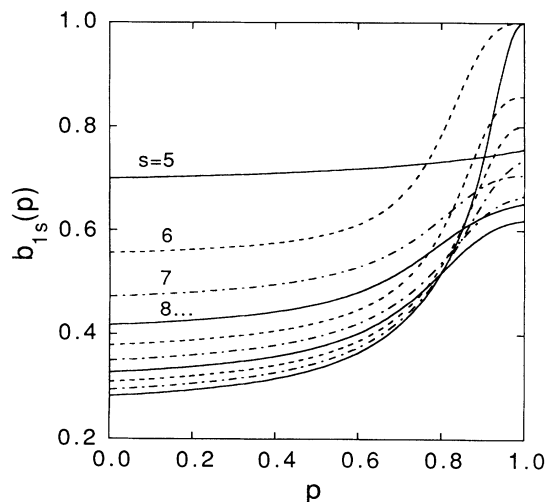
FIG. 13. Exact fraction b_{1s}(p) of unit-mass daughters produced by the fragmentation of clusters of mass s=5, 6, 7, \dots, 14 as a function of the occupancy probability p . This plot illustrates the increasing likelihood of obtaining a very small and a very large daughter, rather than two daughters of comparable masses, as p increases.
