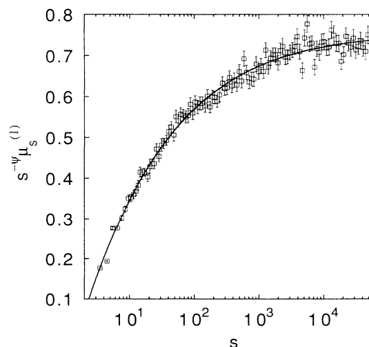
FIG. 2. Computed results (data points) for the ratio of the first moment \mu_s^{(1)} = \sum_{s'=1}^{(s-1)/2} s' c_{s's}(p_c) of the ensemble-average number c_{s's}(p_c) of daughters of mass s' on clusters of mass s to its large- s asymptotic behavior \mu_s^{(1)} \sim s^\psi on an effectively infinite lattice. The solid trace gives a fit with corrections to scaling.
