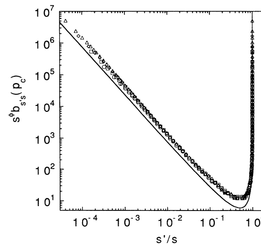
FIG. 5. Scaled daughter distribution s^\phi b_{s's}(p_c) (data points) as a function of the scaled daughter mass s'/s for parent masses s in the same ranges as Fig. 4, with the presumed exact value \phi = \frac{146}{91} . Slight deviations from scaling are evident for very small daughter masses s' (leftmost points for each range of s ). The solid trace gives the corresponding scaling function g(s'/s) for the Bethe lattice [Eq. (6)] with coordination number z = 3 .
