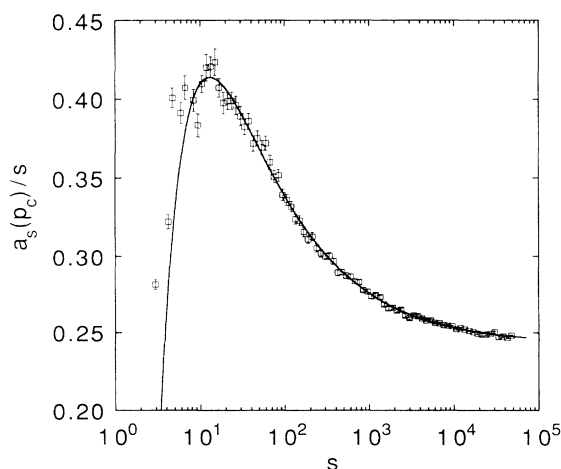
FIG. 1. Computed fraction of fragmenting bonds on two-dimensional ( d=2 ) bond percolation clusters at p=p_c as a function of cluster mass s . The solid trace is a fit to the data involving corrections to scaling.
