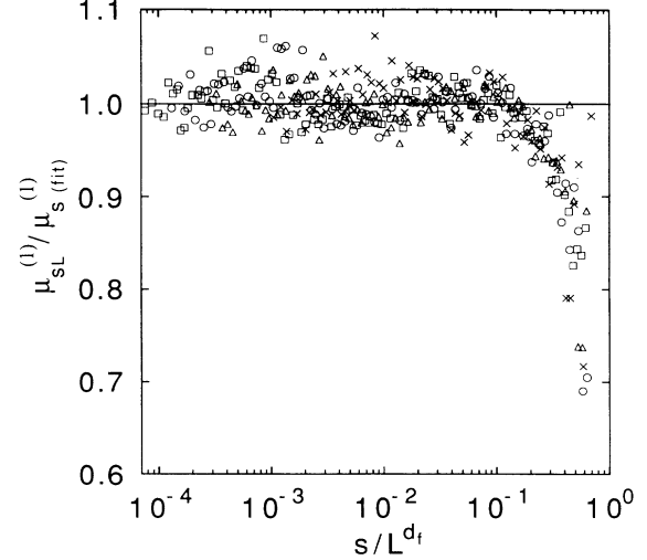
FIG. 7. Ratios of computed first moments at finite L to the fitted first moment on an effectively infinite lattice \mu_{sL}^{(1)}/\mu_{s(\text{fit})}^{(1)} as a function of scaled cluster mass s/L^{d_f} for the same data as Fig. 5, where d_f = \frac{91}{48} is the fractal dimension.
